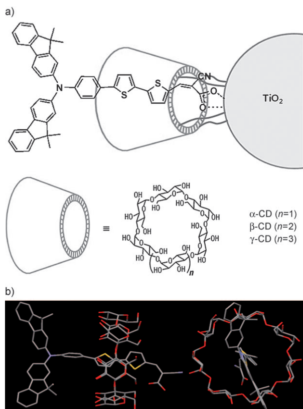
Figure 1. a) The JK-2 sensitizer encapsulated in a cyclodextrin anchored to TiO 2 . b) Energy-minimized structure of JK-2 inside a \beta -cyclodextrin.
