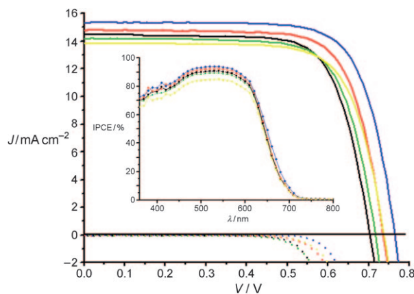
Figure 2. J-V curve and IPCE spectra (inset) of JK-2 (black line), JK-2/DCA (red line), \alpha -CD/JK-2 (green line), \beta -CD/JK-2 (blue line), and \gamma -CD/JK-2 (yellow line). The dark current/bias potential relationship is shown as dotted curves.
